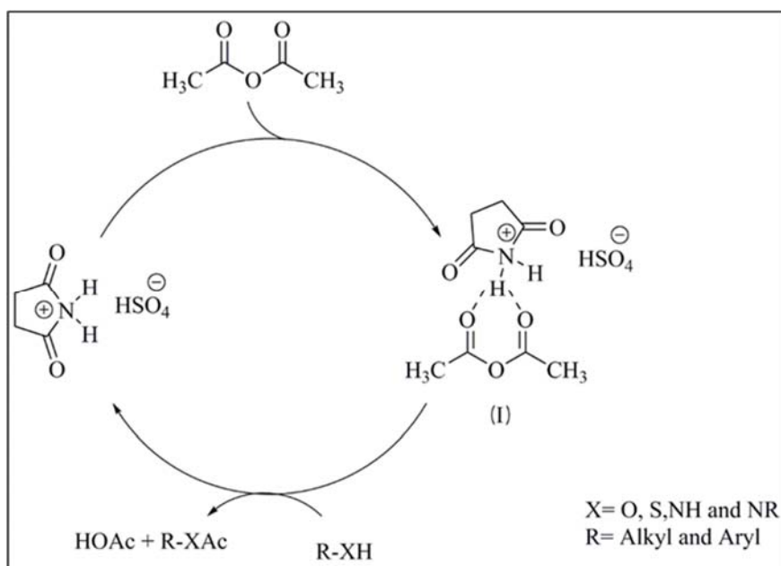
Scheme 2. The plausible mechanism of the reaction.
