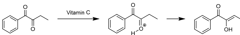
Scheme 2. Enolization of \alpha - diketones in the presence of vitamin C.
