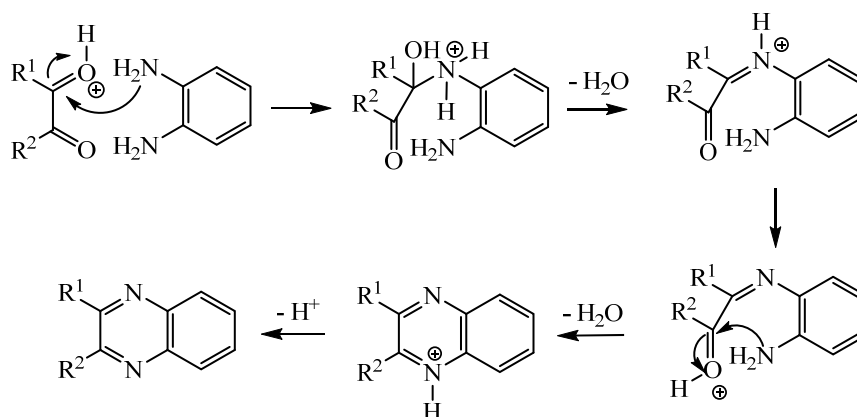
Scheme 3. The plausible mechanism for synthesis of quinoxaline derivatives.
