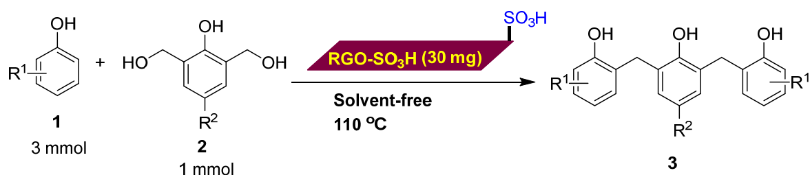
Scheme 2. Optimized reaction conditions for synthesis of trisphenols in the presence of RGO-SO 3 H.
