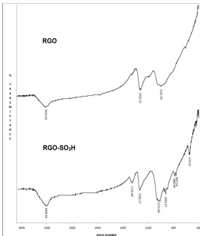
Fig. 3. A comparison between the FT-IR spectrum of RGO and RGO-SO 3 H.
