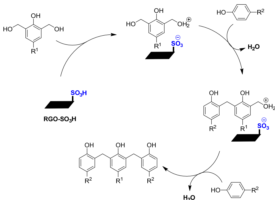
Scheme 3. Proposed reaction mechanism for synthesis of trisphenols using RGO-SO 3 H catalyst.
