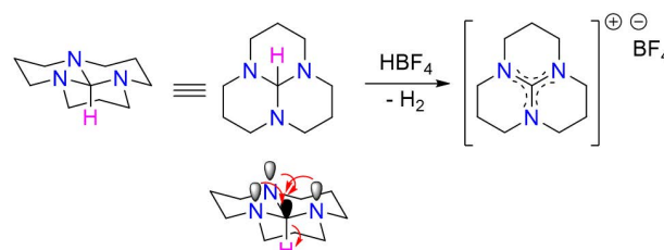
Scheme 2. Anomeric effect causes to hydrogen releasing from the tricyclic orthoamide
